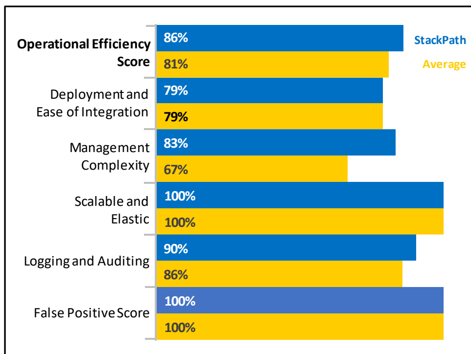
Figure 3. Validation of Operational Efficiency for StackPath Web Application Firewall
