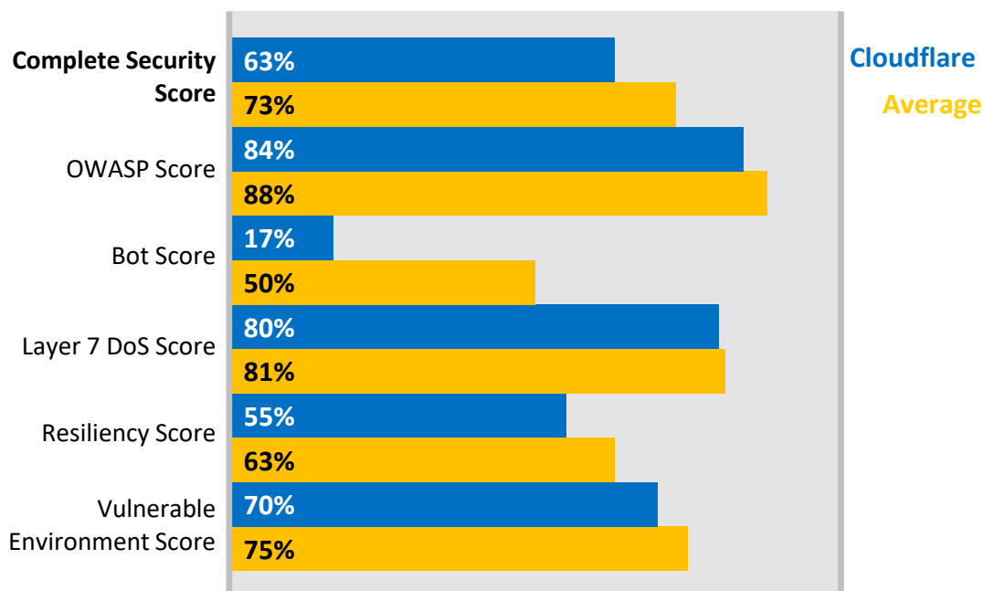
Figure 2. Security Validation Results for Cloudflare Business Web Application Firewall
