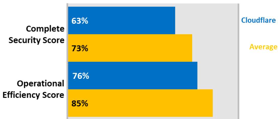
Figure 1. Overall Validation Results for Cloudflare Business Web Application Firewall
