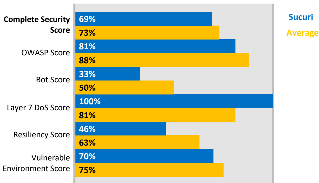
Figure 2. Security Validation Results for Sucuri's Web Application Firewall
