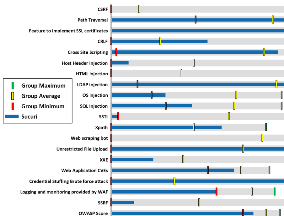
Figure 3. OWASP Score Visual
